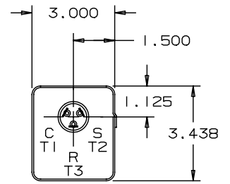
TERMINAL BOX (QUICK-CONNECT TERMINALS)
