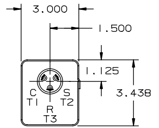
TERMINAL BOX (QUICK-CONNECT TERMINALS)
