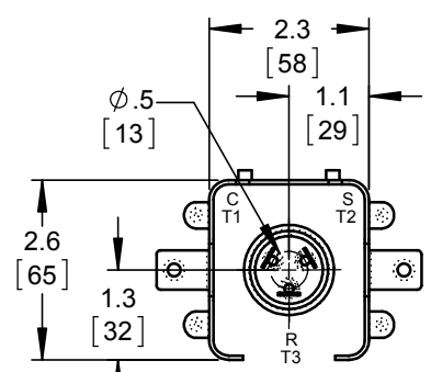
TERMINAL BOX (QUICK CONNECT TERMINALS)
